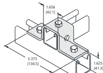
UL-1047 Conector "U" 5 orificios Five hole "U" support
