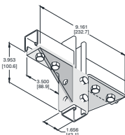
UL-2348 Conector de 2 alas 10 orificios Ten hole double wing gusseted connection
