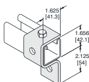
UL-1046A Conector de copa 3 orificios Three hole cup supportplate
