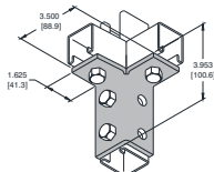
UL-2224 Conector de esquina doble 6 orificios Six hole double corner connection
