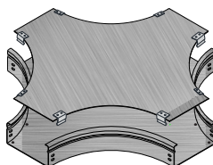
"X" HORIZONTAL HORIZONTAL CROSS
