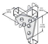
UL-2235 Conector angular 90° tipo trapezio 5 orificios Five hole gussetted three way shelf angle
