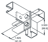
UL-1038 Conector angular 90° derecho 3 orificios Three hole (right hand) offset bent angle
