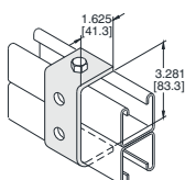
UL-1044 Conector "U" 4 orificios Four hole clevis
