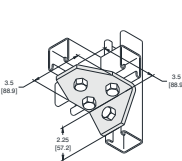
UL-1579 Conector angular 90° tipo trapezio 4 orificios Four hole gusseted three way shelf angle
