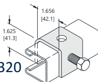
UL-1043A Conector "U" 6 orificios Six hole "U" support
